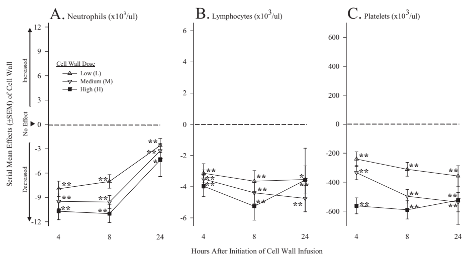
Figure 3 Serial mean effects ( \pm SEM) of low (L), medium (M), or high (H) cell-wall doses compared with controls (phosphate-buffered saline; see Methods regarding calculation of the effects) on circulating neutrophil, lymphocyte, and platelet concentrations at 4, 8, and 24 hours after the initiation of challenges (designated on the x axis as 4, 8, or 24). Significant effects are designated by asterisks (* \leq 0.05; ** \leq 0.0001).
