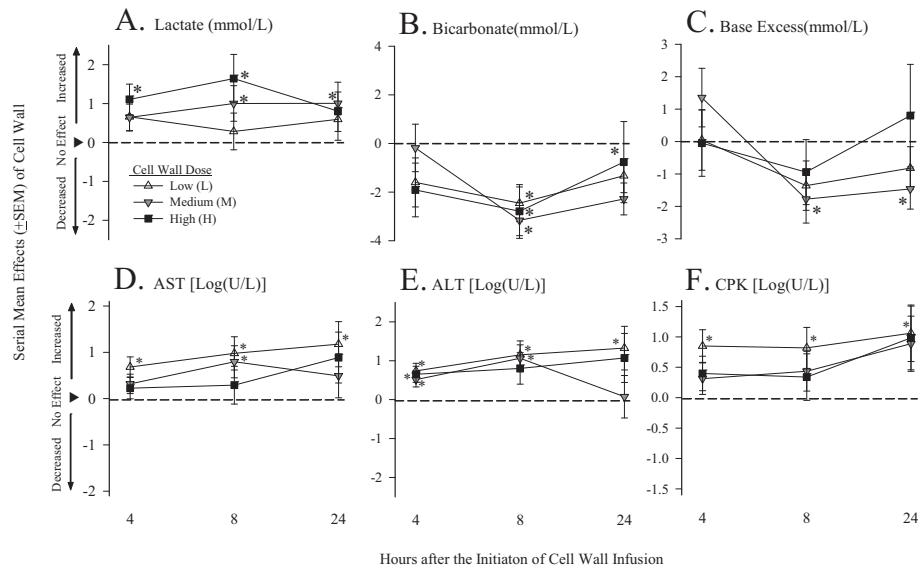
Figure 5 Serial mean effects ( \pm SEM) of low (L), medium (M), or high (H) cell-wall doses compared with controls (phosphate-buffered saline; see Methods regarding calculation of the effects) on lactate, bicarbonate, base excess, aspartate and alanine aminotransaminases (AST and ALT, respectively), and creatine phosphokinase (CPK) at 4, 8, and 24 hours after the initiation of challenges (designated on the x axis as 4, 8, or 24). Significant effects are designated by the asterisks (* \leq 0.05 ; ** \leq 0.0001 ).
